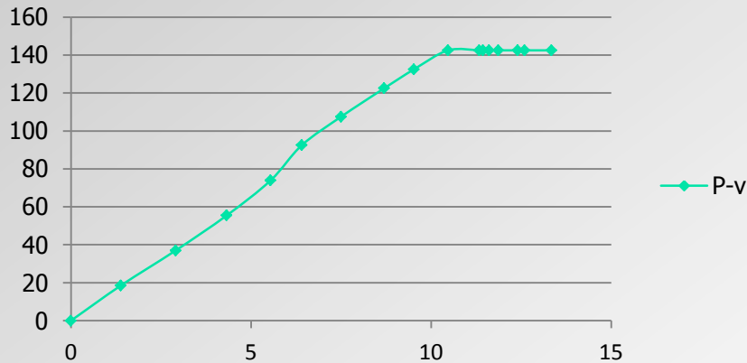
Load P (KN) - displacement v (mm)
